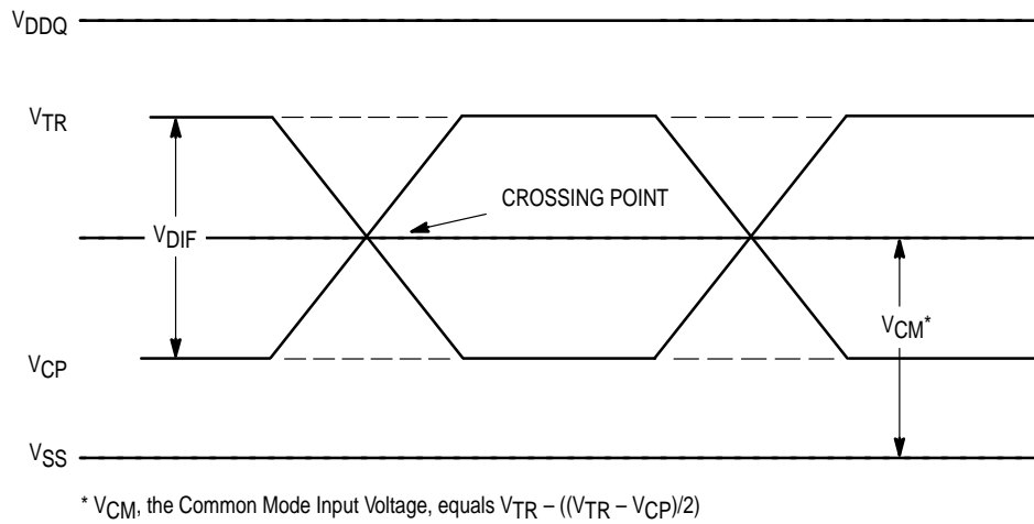
Figure 3. Differential Inputs/ Common Mode Input Voltage
