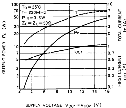
OUTPUT POWER, TOTAL CURRENT, FIRST CURRENT VS. SUPPLY VOLTAGE
