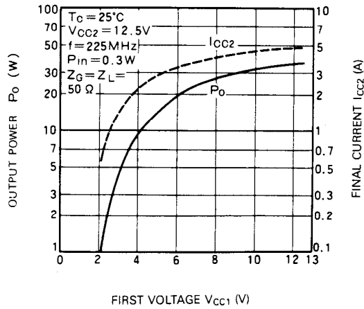
OUTPUT POWER, FINAL CURRENT, VS. FIRST VOLTAGE
