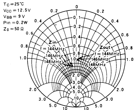
INPUT IMPEDANCE, OUTPUT IMPEDANCE VS. FREQUENCY
