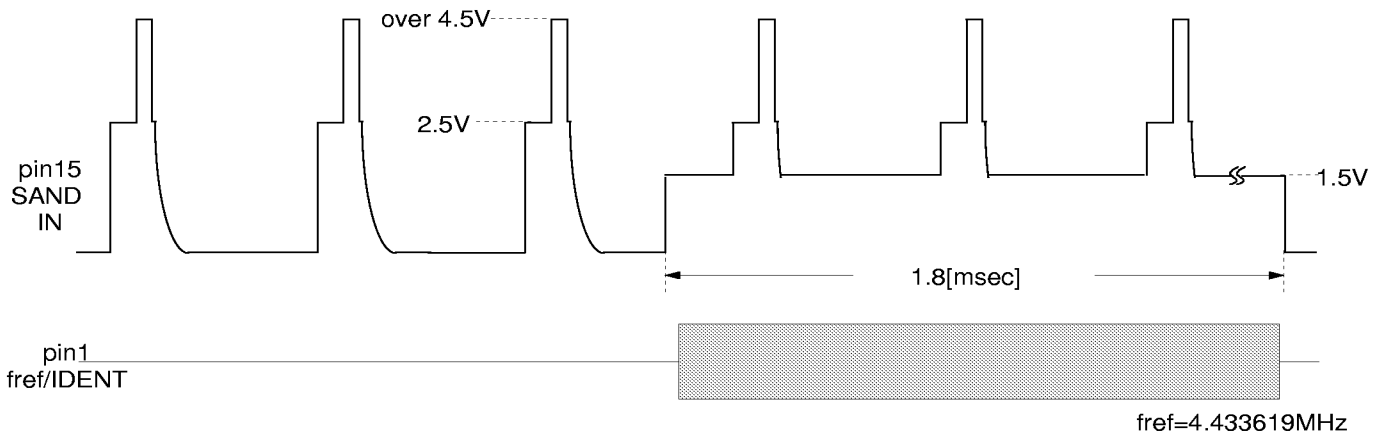
fig.5 sandcastle pulse and fref signal
