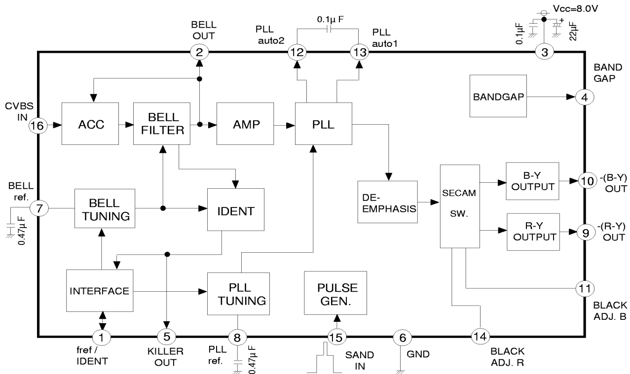
fig.1 M52325AP block diagram
