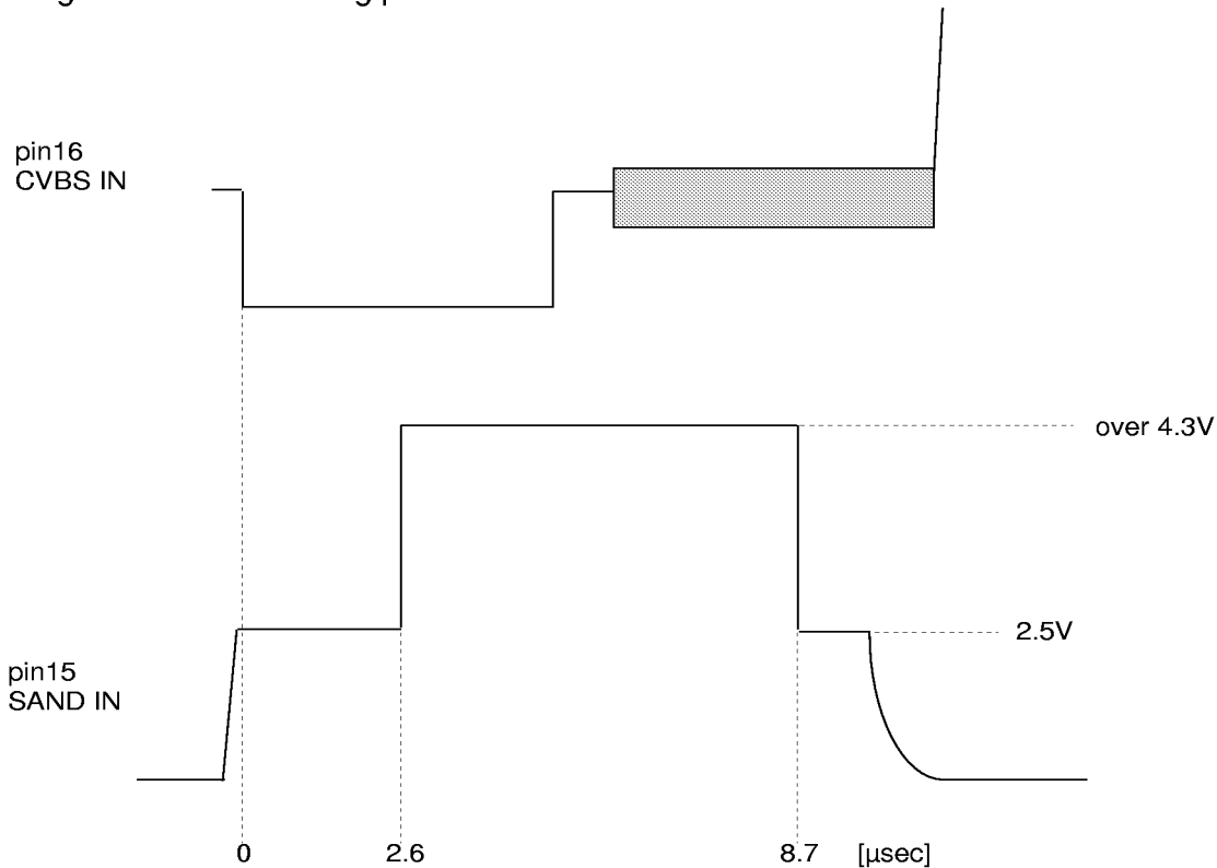
fig.4 sandcastle pulse
