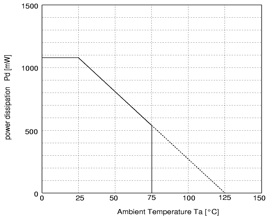
fig.3 package thermal derating curve ( maximum rating )
