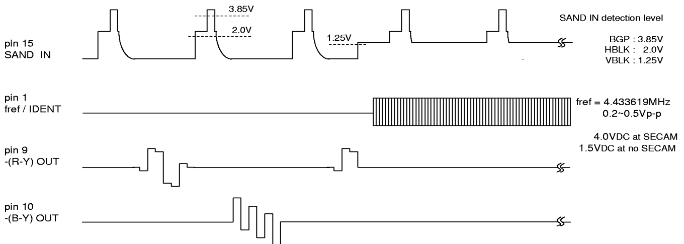
fig.2 timing waveforms
