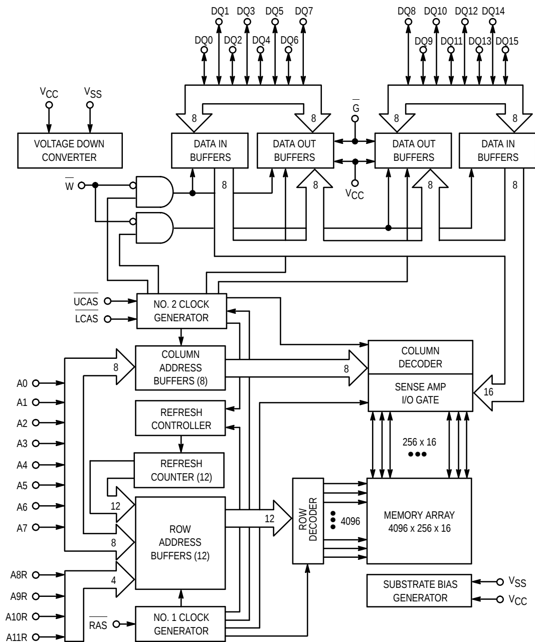
MCM516160B BLOCK DIAGRAM 1M x 16, 4096 CYCLE REFRESH
