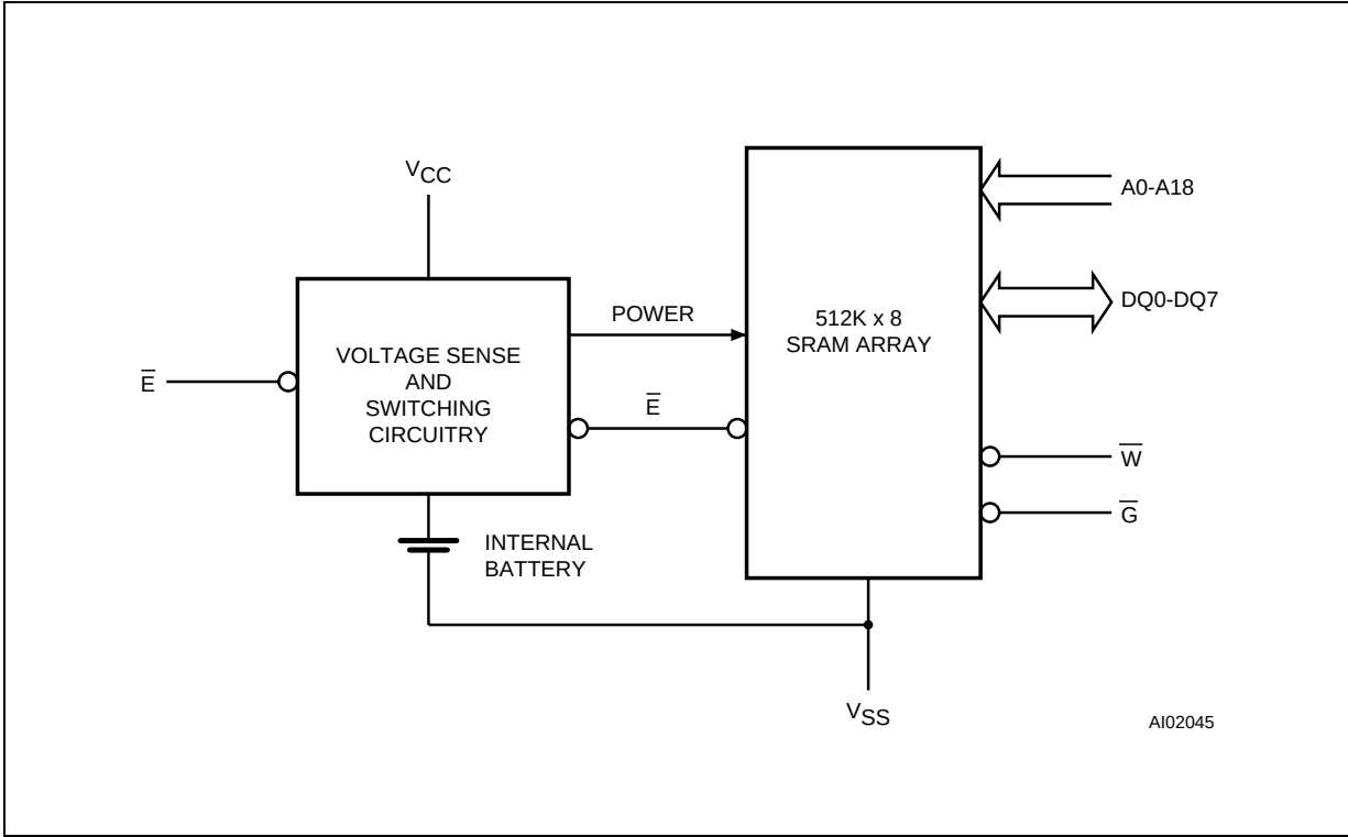
Figure 3. Block Diagram
