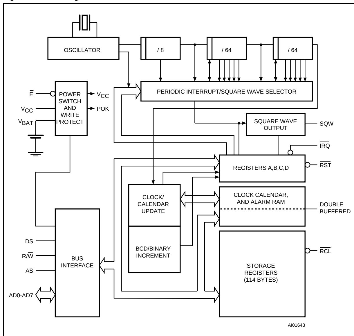
Figure 3. Block Diagram
