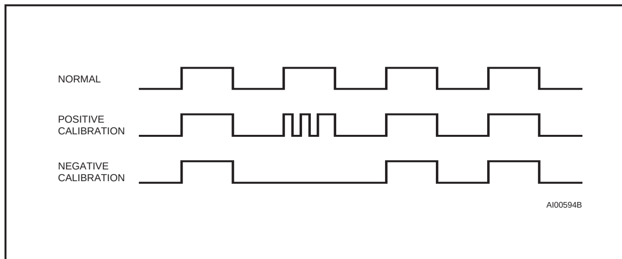
Figure 9. Clock Calibration
