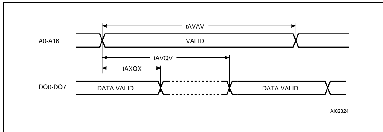
Figure 6. Address Controlled, Read Mode AC Waveforms
