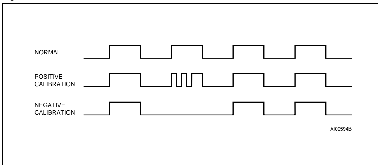
Figure 9. Clock Calibration
