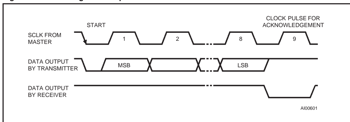
Figure 7. Acknowledgement Sequence
