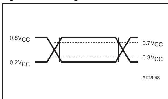
Figure 4. AC Testing Load Circuit
