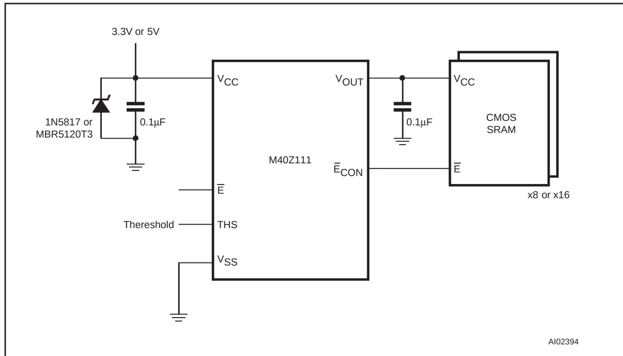
Figure 3. Hardware Hookup
