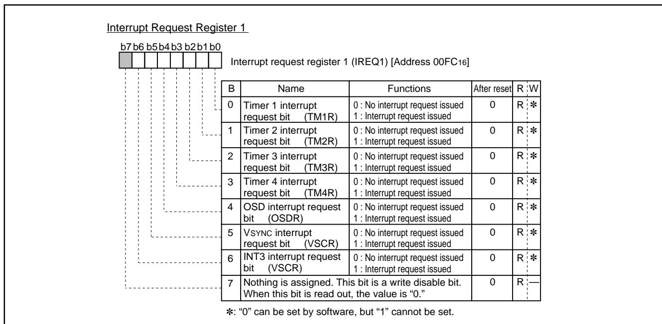
Fig. 10. Interrupt Request Register 1
