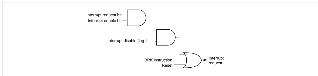
Fig. 9. Interrupt Control
