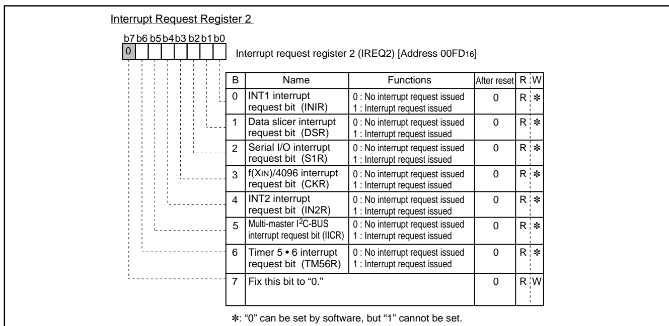
Fig. 11. Interrupt Request Register 2
