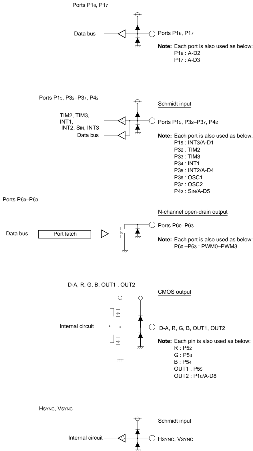
Fig. 53. I/O pin block diagram (2)
