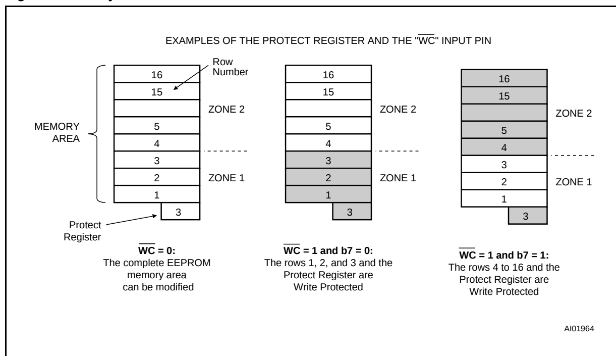
Figure 9. Memory Protection
