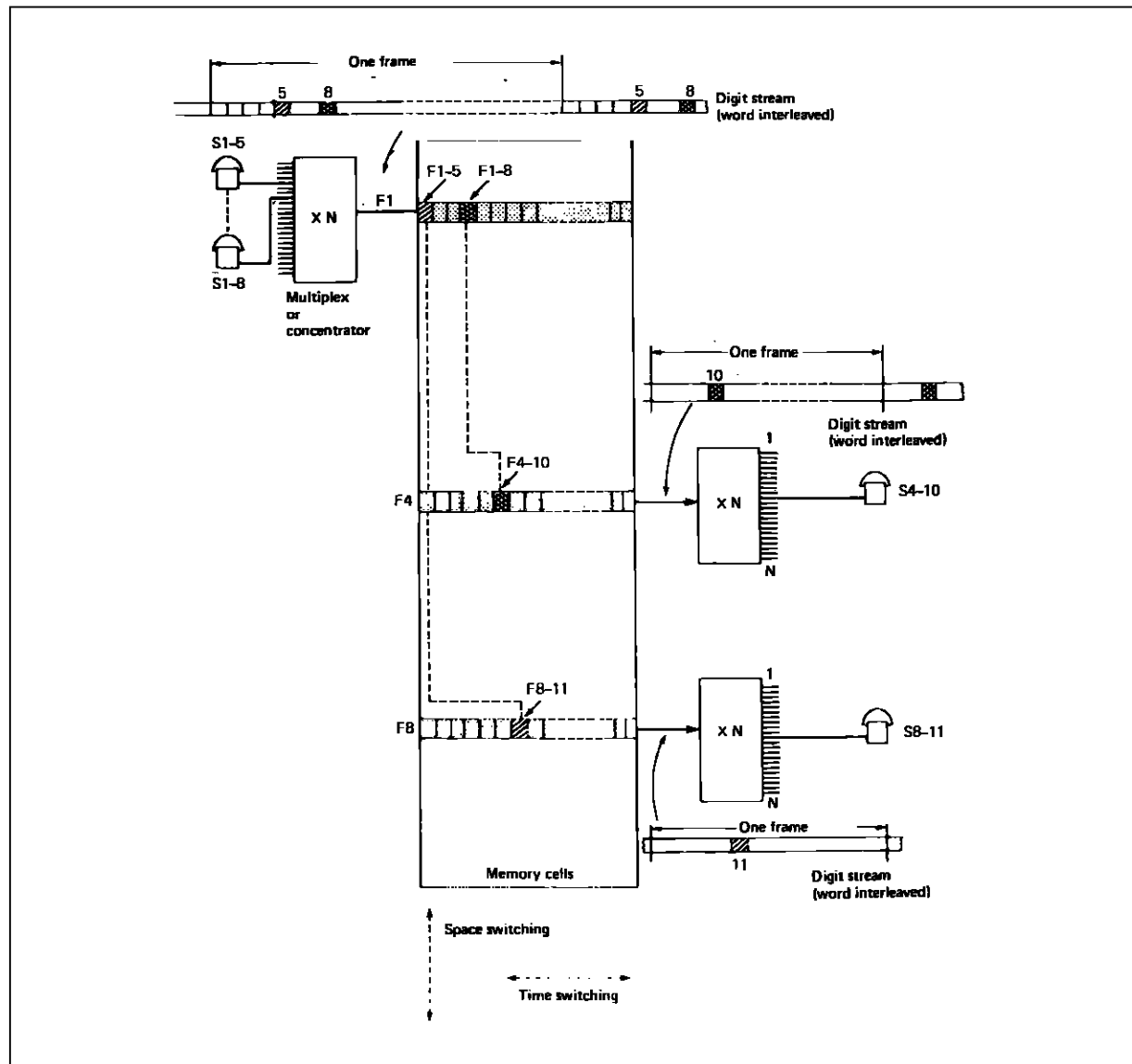
Figure 1.6 : Space-and-Time-switching Digitally encoded Signals.
