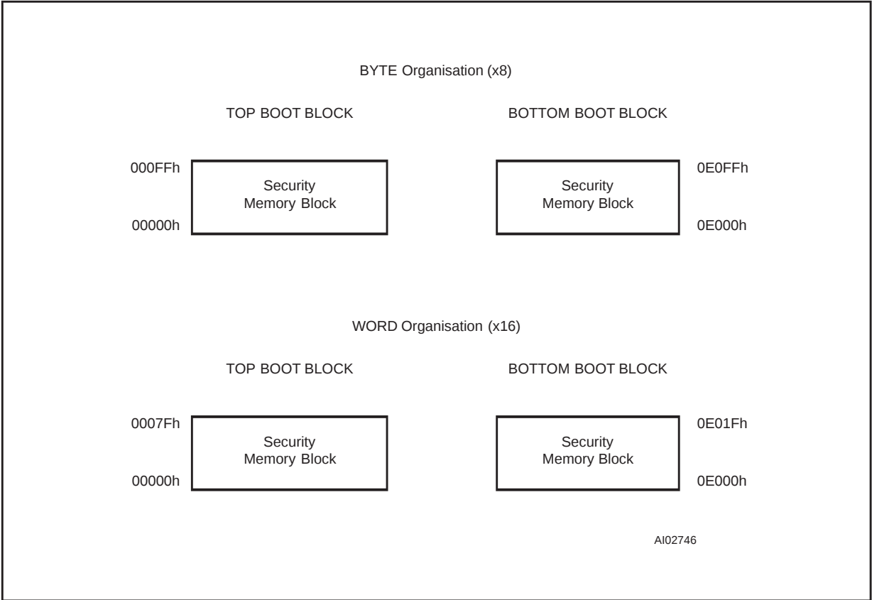
Figure 14. Security Block Address Table
