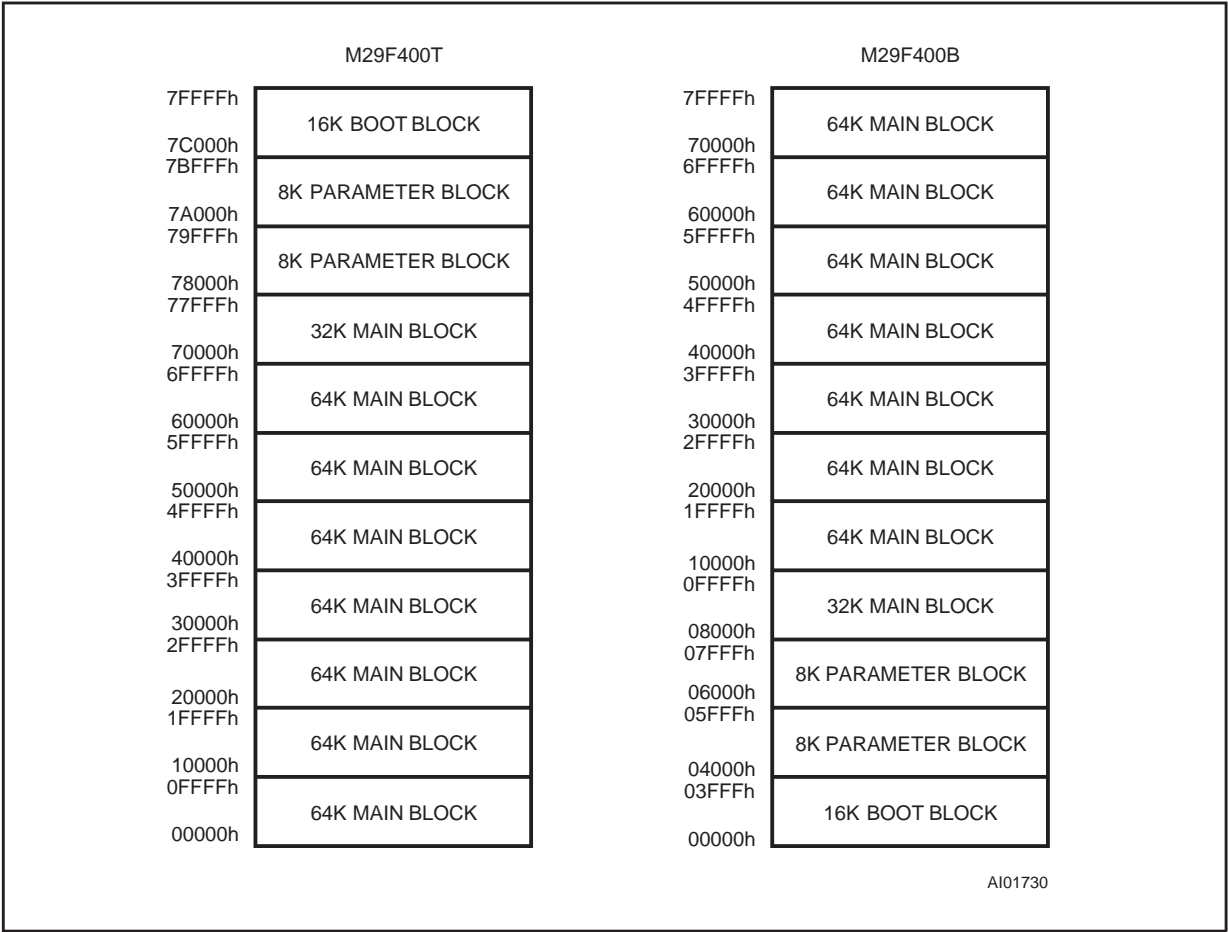
Figure 3. Memory Map and Block Address Table (x8)
