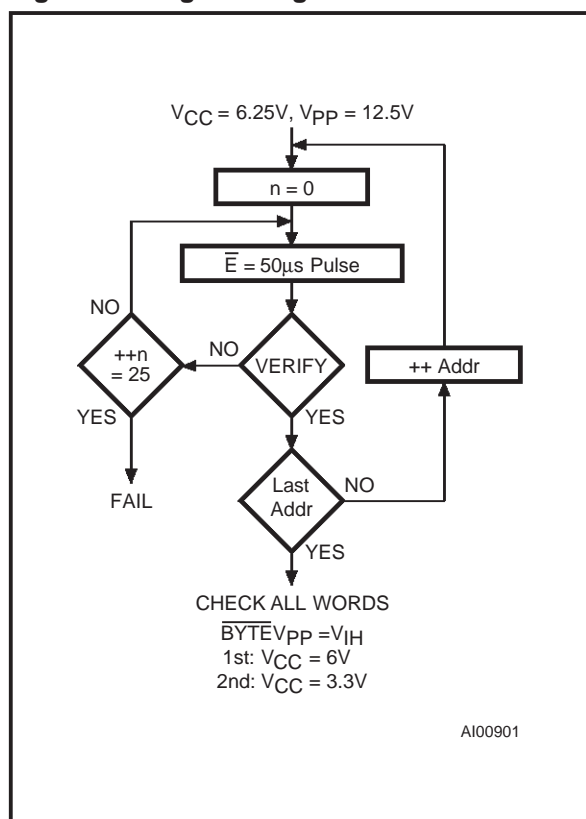
Figure 9. Programming Flowchart
