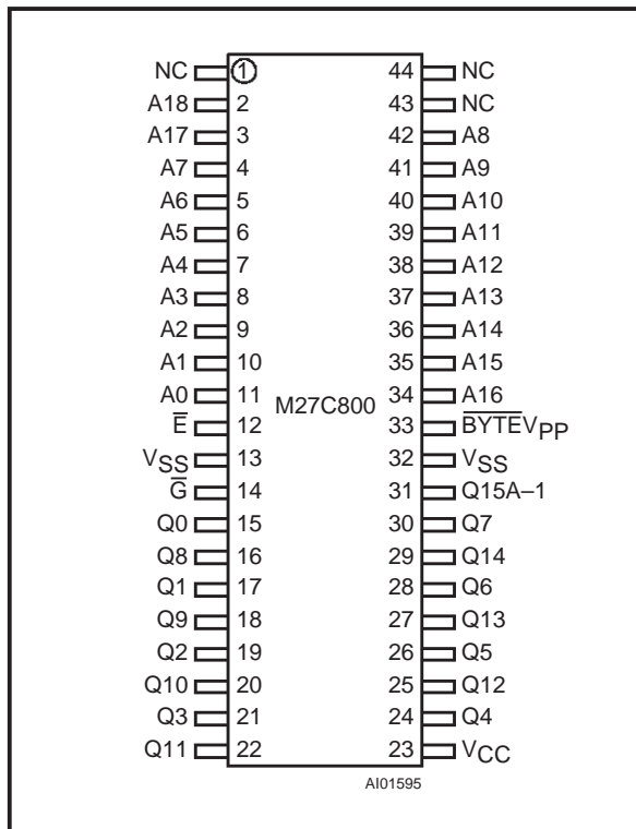
Figure 2B. SO Pin Connections
