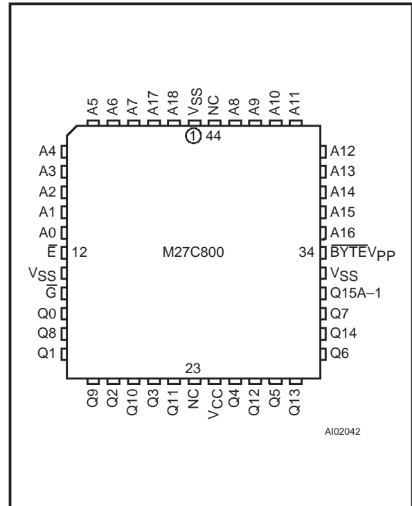
Figure 2C. LCC Pin Connections
