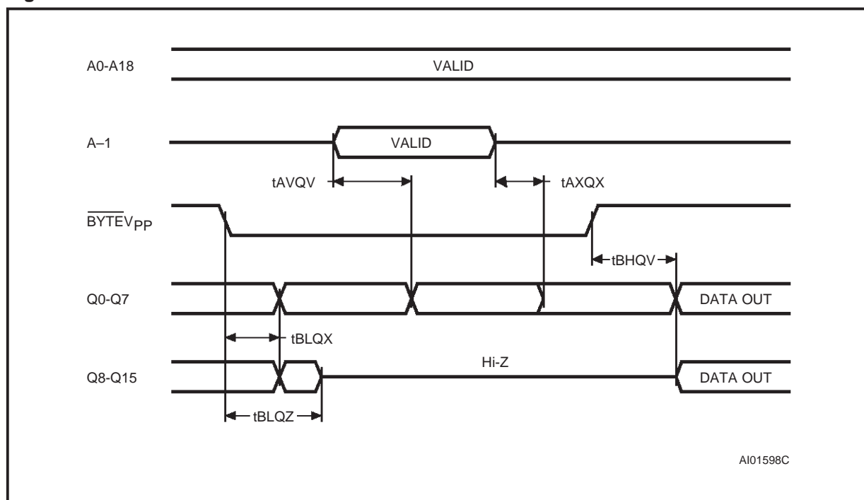
Figure 7. BYTE Transition AC Waveforms
