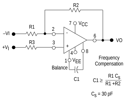
Figure 14. Single-Pole Compensation
