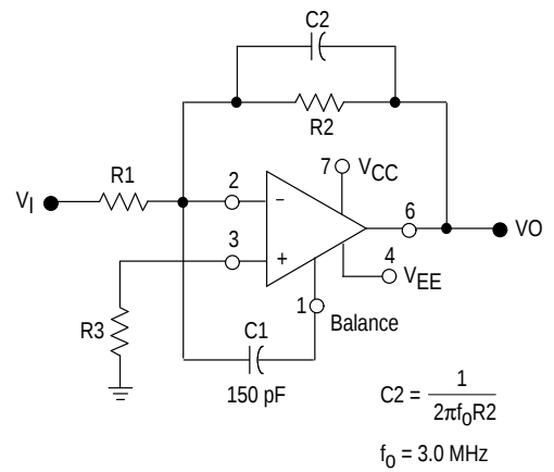
Figure 15. Feedforward Compensation
