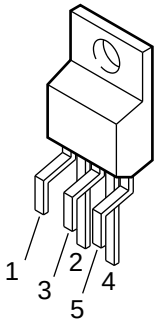
BENT AND STAGGERED LEADS LB03 TYPE
