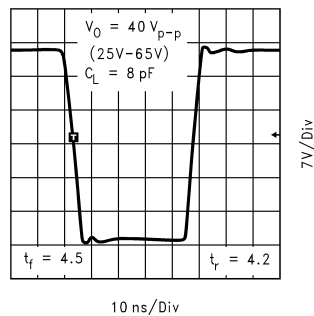
FIGURE 5. Pulse Response
