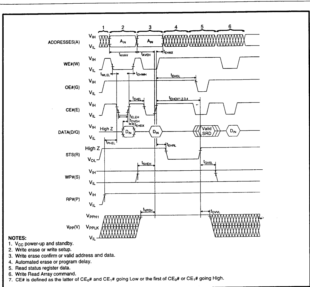
Figure 20. AC Waveform for CE\# -Controlled Write Operations
