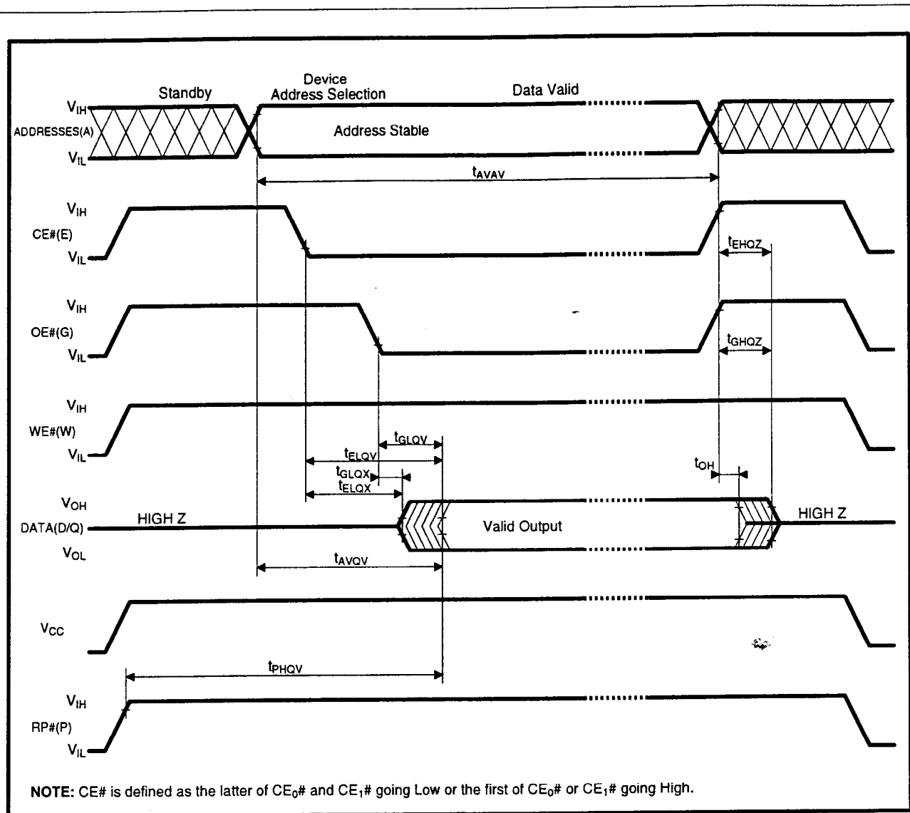
Figure 17. AC Waveform for Read Operations
