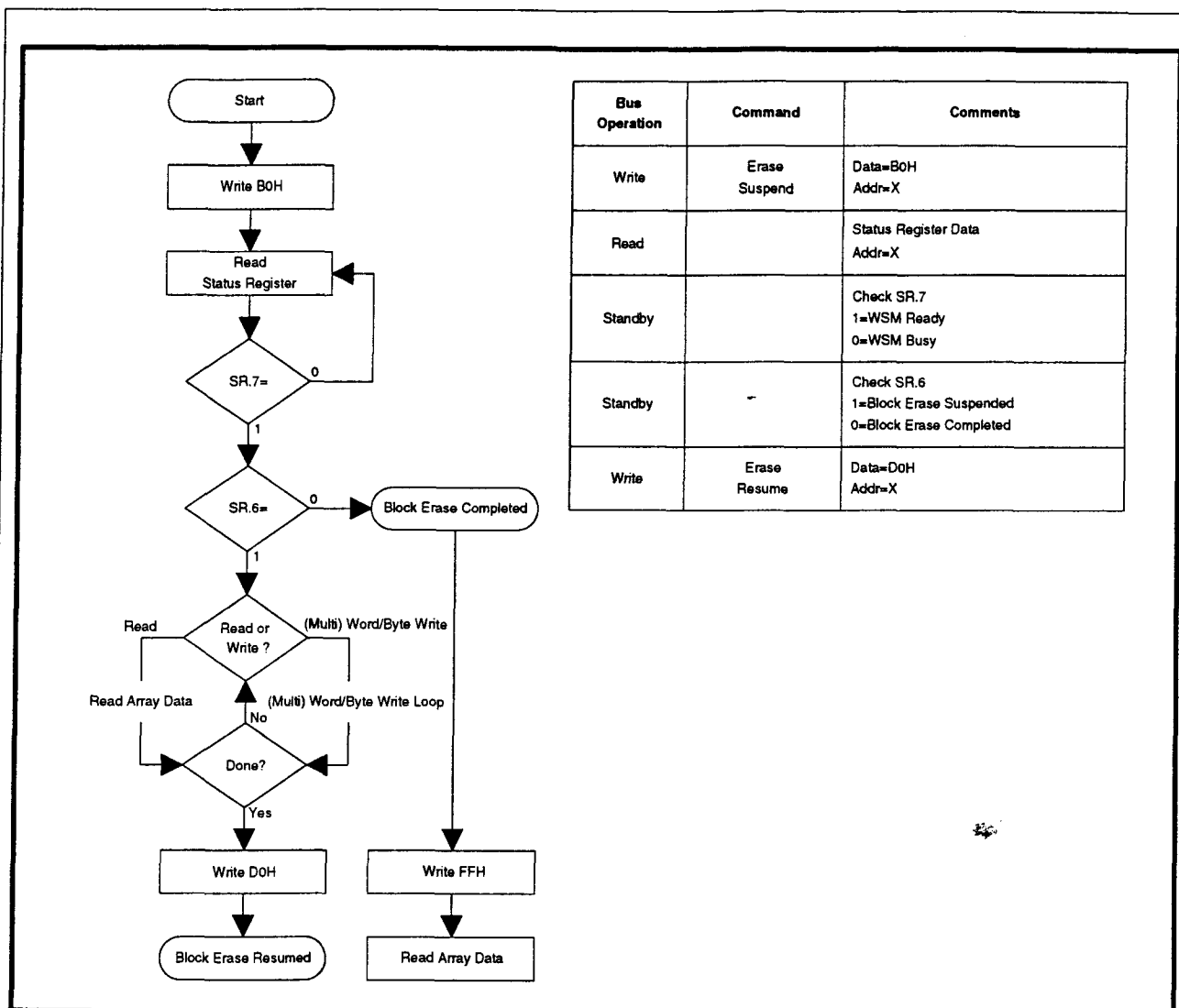
Figure 10. Block Erase Suspend/Resume Flowchart
