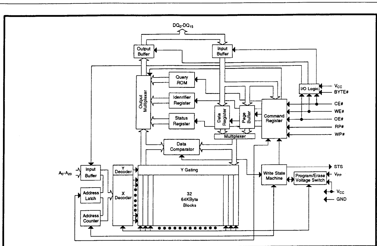
Figure 1. Block Diagram
