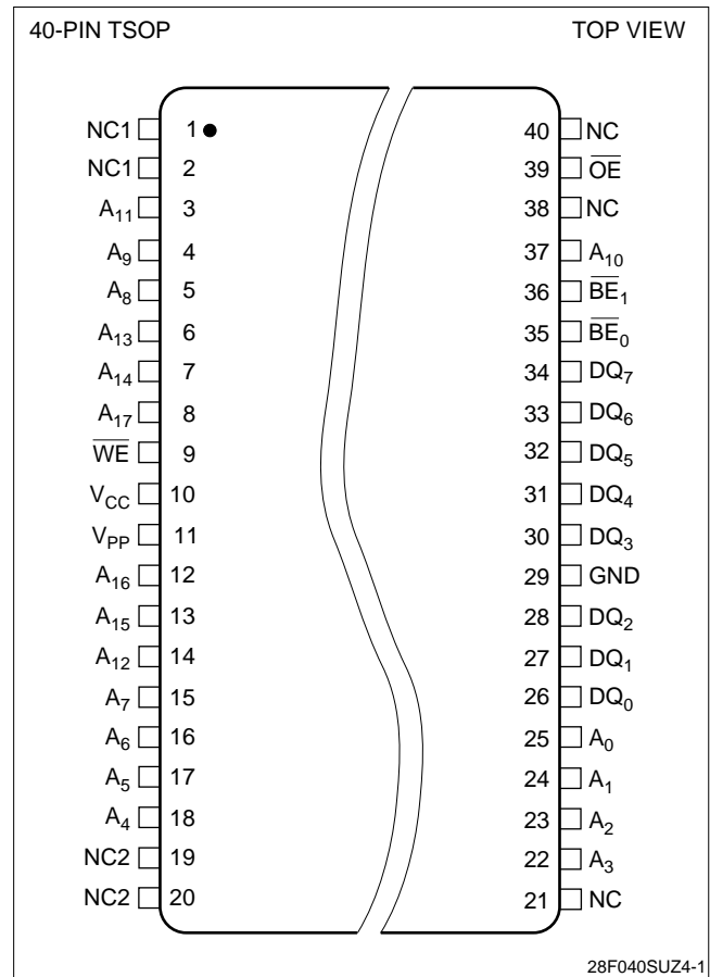
Figure 1. TSOP Configuration
