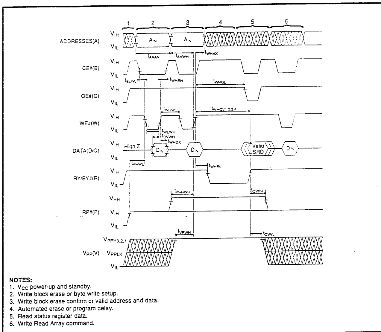
Figure 19. AC Waveform for WE#-Controlled Write Operations
