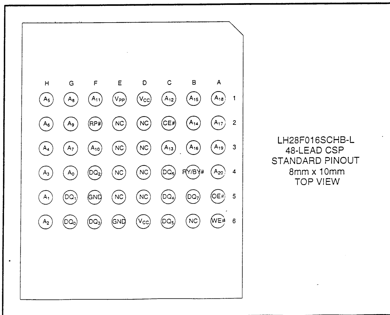
Figure 5. CSP 42-Lead Pinout
