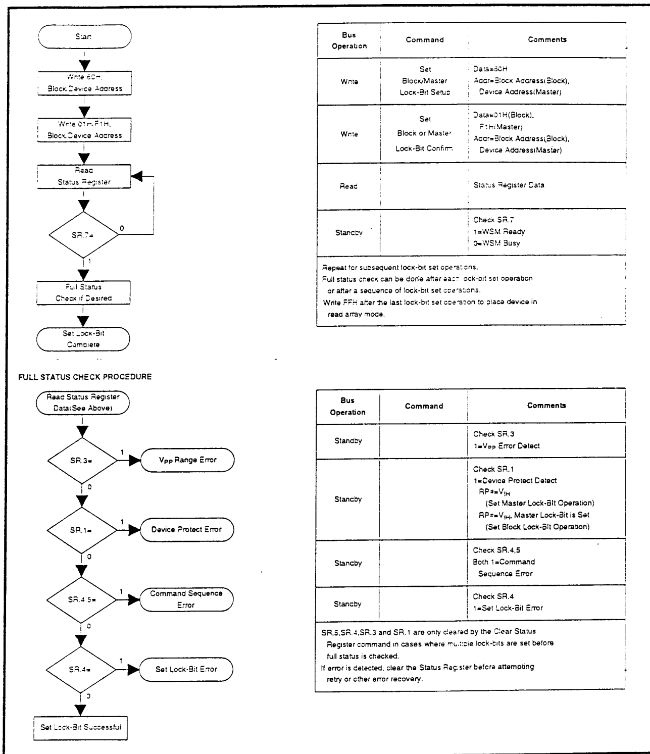
Figure 12. Set Block and Master Lock-Bit Flowchart
