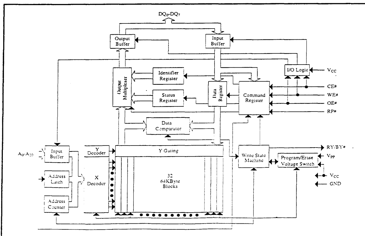
Figure 1. Block Diagram
