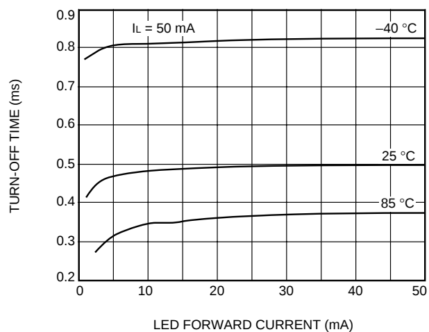
B. Turn-Off Time vs. LED Current (LH1531)
