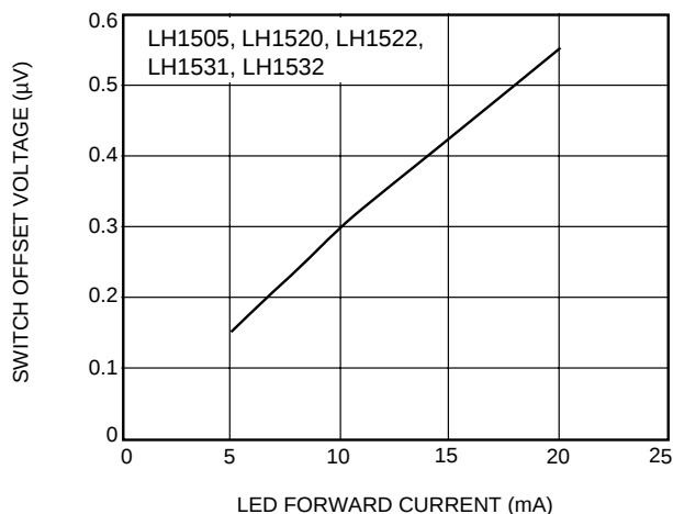
A. Switch Offset Voltage vs. LED Current
