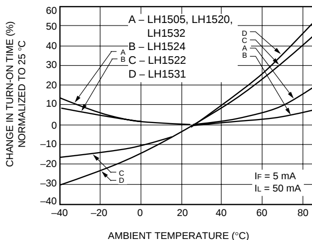
C. Turn-On Time vs. Temperature
