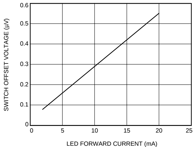
B. Switch Offset Voltage vs. LED Current (LH1544)
