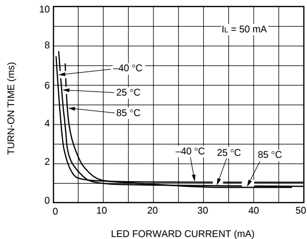
B. Turn-On Time vs. LED Current (LH1522)
