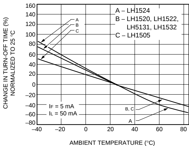
E. Turn-Off Time vs. Temperature
