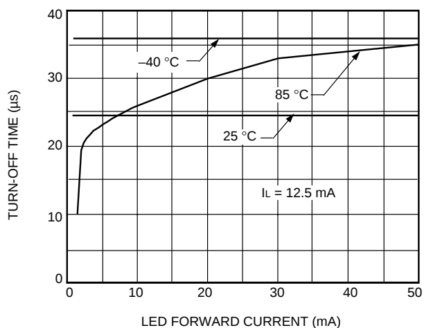
C. Turn-Off Time vs. LED Current (LH1544)
