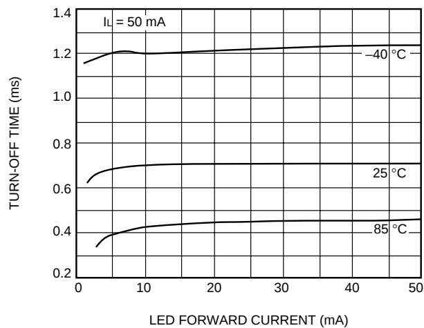
F. Turn-Off Time vs. LED Current (LH1505, LH1520, LH1522, LH1532)
