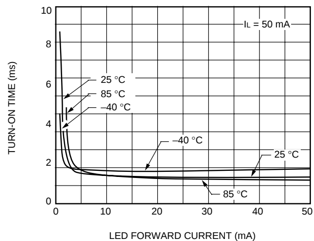
C. Turn-On Time vs. LED Current (LH1524)
