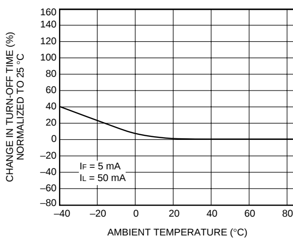
F. Turn-Off Time vs. Temperature (LH1544)
