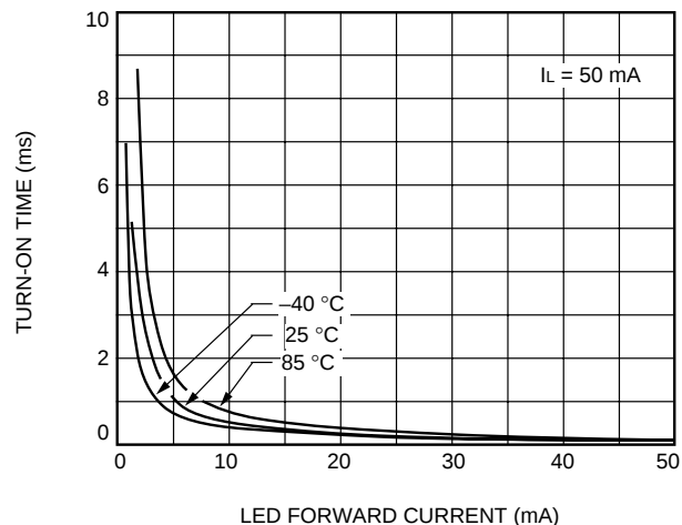
D. Turn-On Time vs. LED Current
