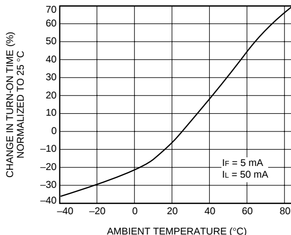
D. Turn-On Time vs. Temperature (LH1544)
