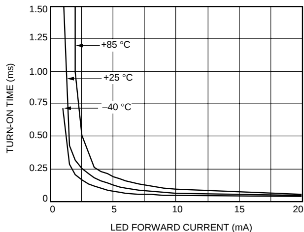
E. Turn-On Time vs. LED Current (LH1544)
