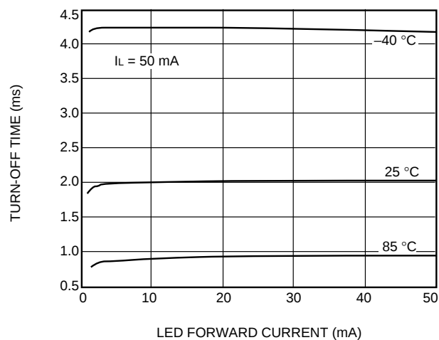
A. Turn-Off Time vs. LED Current (LH1524)
