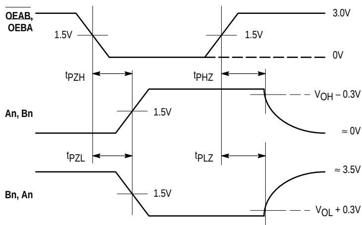
WAVEFORM 2 – OExx to An/Bn OUTPUT ENABLE AND DISABLE TIMES
