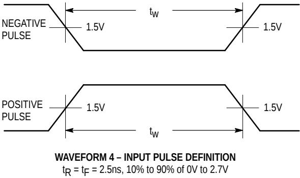
Figure 2. AC Waveforms
