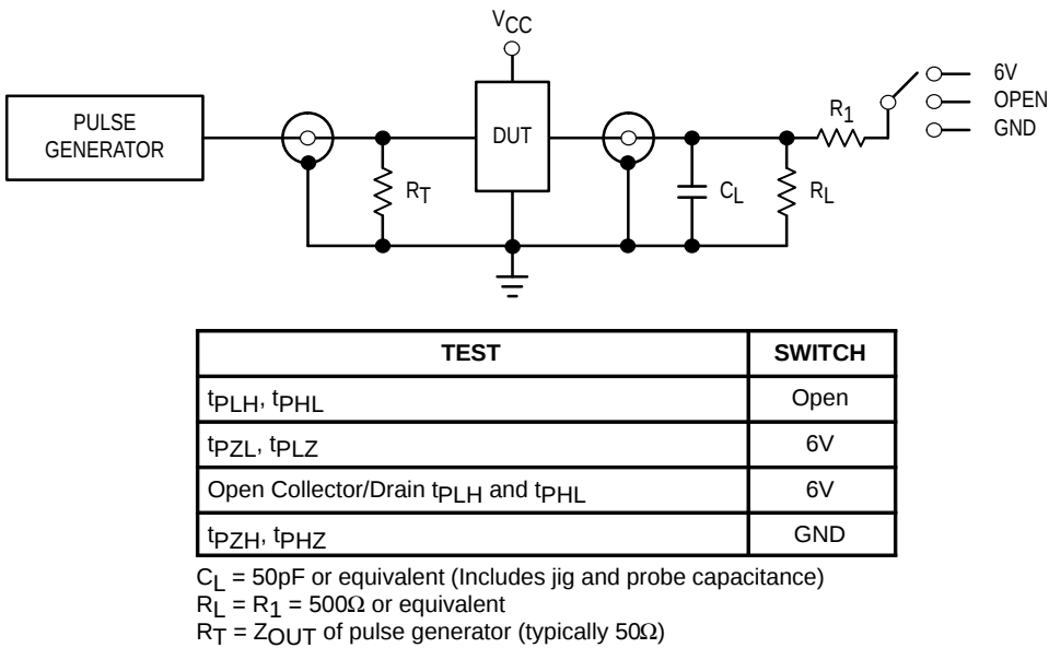
Figure 3. Test Circuit
