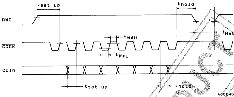
Figure 1 Command Input
