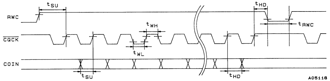
Figure 1 Command Input
