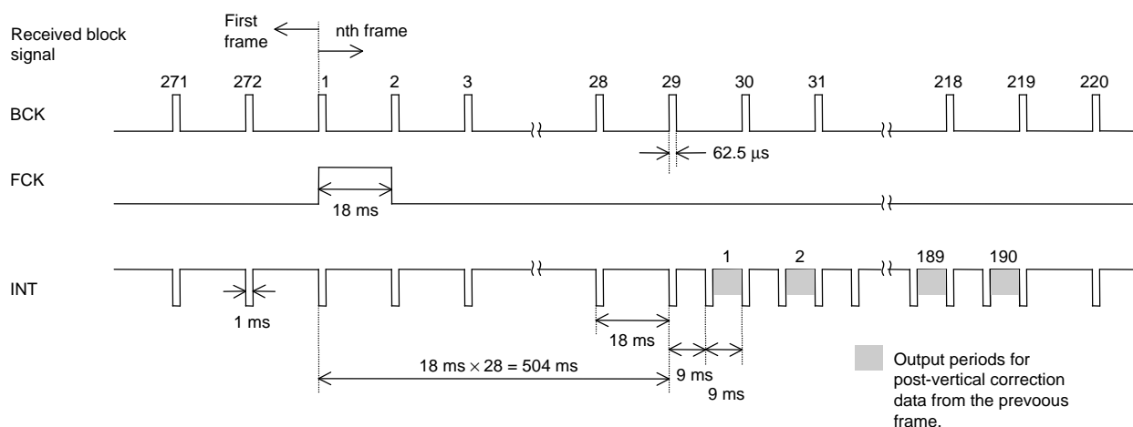
Figure 4 Post-Vertical Correction Data Output Timing
