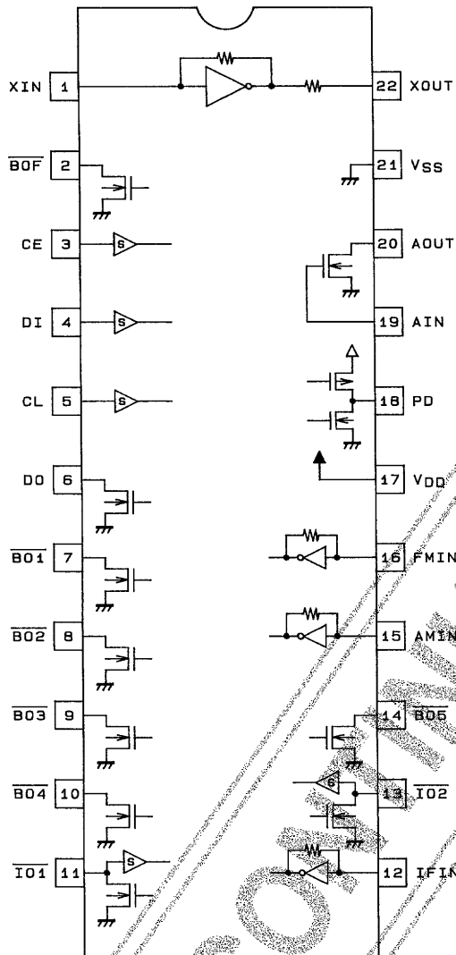
Top view
