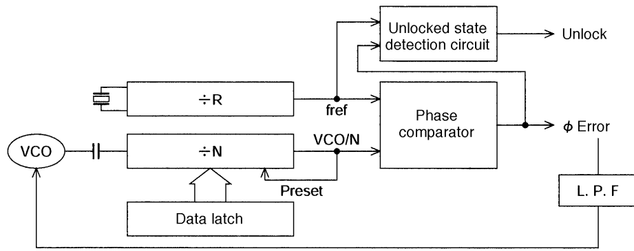
Figure 2 Circuit Structure
