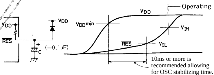
Figure 3. Reset Circuit
