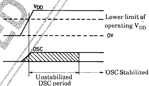
Figure 2. Stabilization Time
