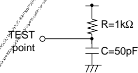
Figure 5 Timing Load
