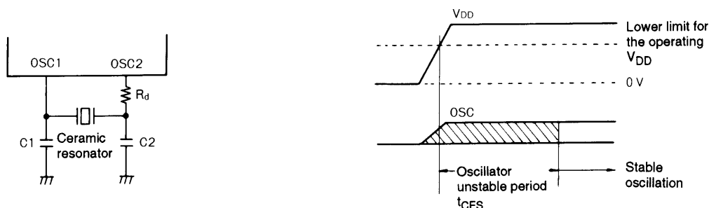
Figure 2 Ceramic Oscillator Circuit
