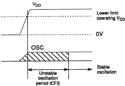
Fig. 3 Oscillator Stabilization Period
