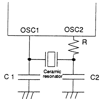
Fig. 3 Ceramic Oscillator
