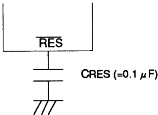
Fig. 4 Reset Circuit
