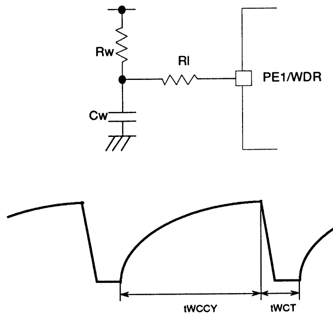
Fig. 8 Watchdog Timer Waveform
