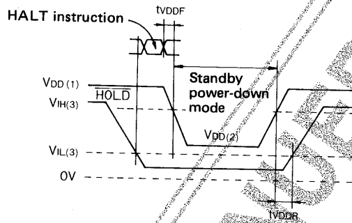
Fig. 1 Standby mode timing
