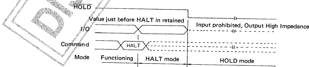
Fig. 4-2 Mode change from HALT mode to HOLD mode
