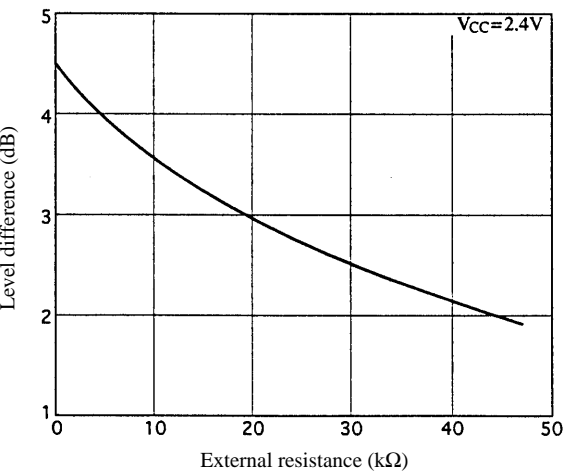
Graph 2. Transmitter Gain Change Level vs. External Resistance
