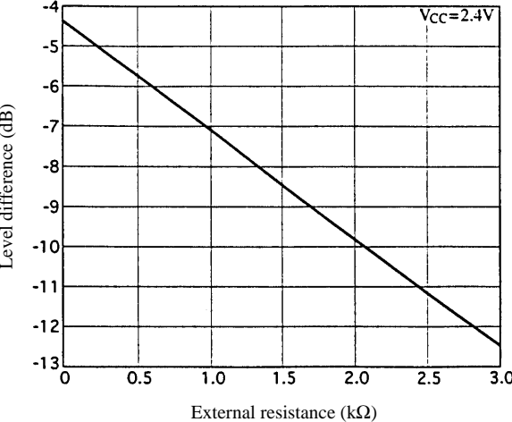
Graph 3. Receiver Gain Change Level vs. External Resistance
