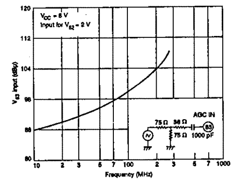
AGC frequency response
