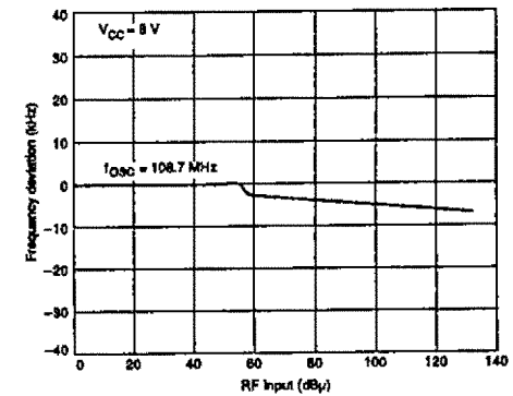
Oscillator frequency deviation vs. Input
