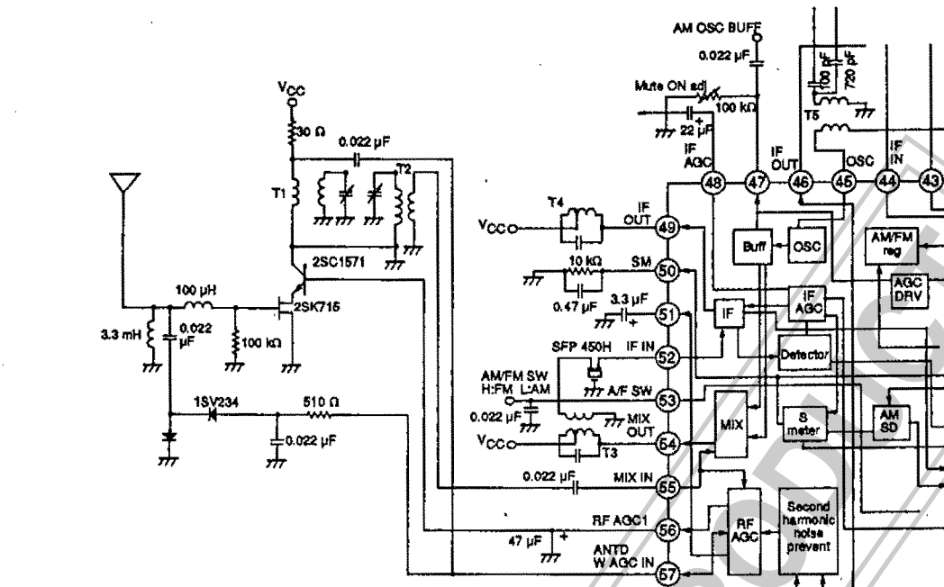
Figure 21. AGC stage
