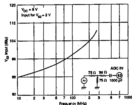
Figure 3. Input characteristic
