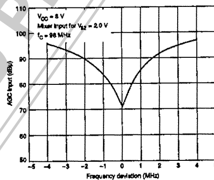
Figure 3. Input characteristic
