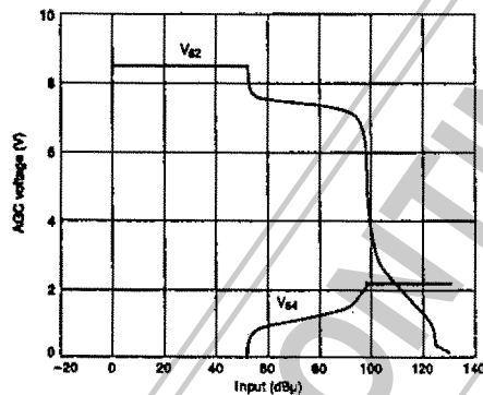
The pin-diode driver operates when the voltage on pin 62 is equal to or less than approximately (V_{cc} - 1) V. The impedance of the pin diode decreases as the current flowing through it increases. The voltage on the second gate of the FET also drops, decreasing the FET's transconductance, g_m . This attenuates the input signal by approximately 30 to 40 dB as shown in figure 2.
