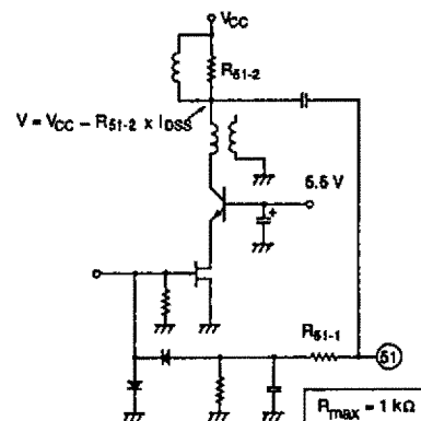
Figure 28. AGC ON level adjustment
