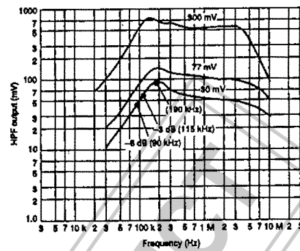
Pin 8 output vs. frequency (1)
