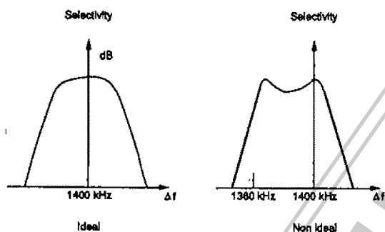
Figure 32. Tracking characteristic
