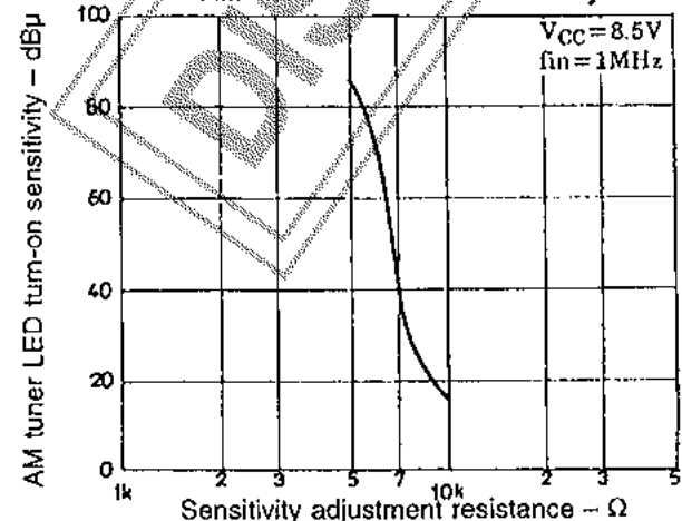
AM TU LED Turn-on Sensitivity
