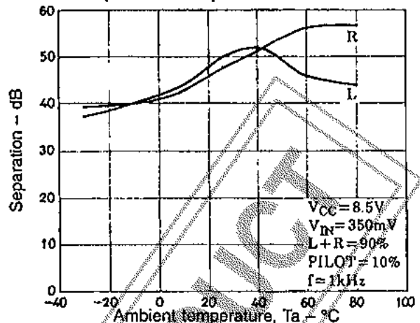
MPX Separation Temperature Characteristics
