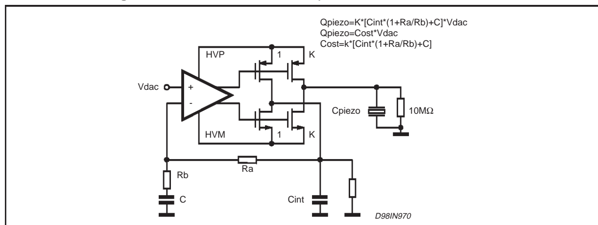
Figure 1. Charge Mode Configuration (only a suggestion, the application is completely free according with Electrical Characteristics).
