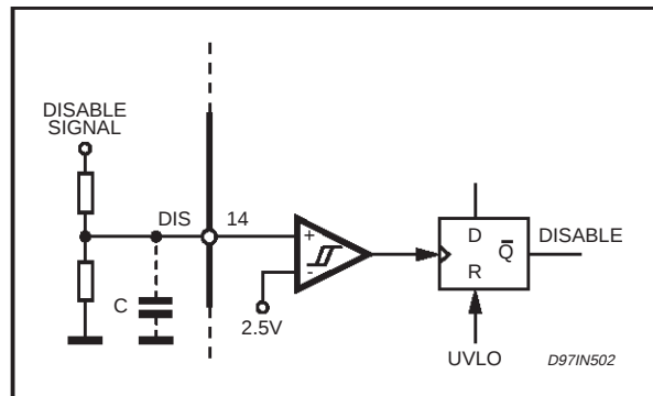
Figure 28. Disable (Latched)
