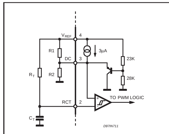
Figure 22. Duty cycle control.
