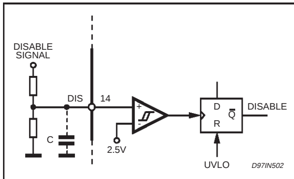
Figure 29. Disable (Latched).
