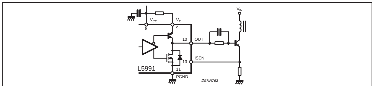
Figure 37. Bipolar transistor driver.
