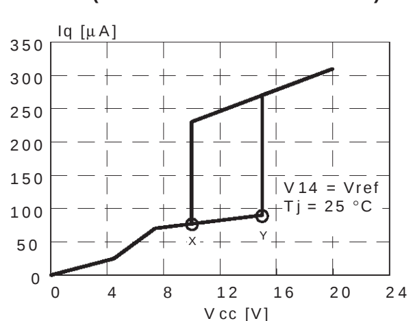
Figure 2. L5991 - Quiescent current vs. input voltage (after disable). (X = 7.6V and Y = 8.4V for L5991A)
