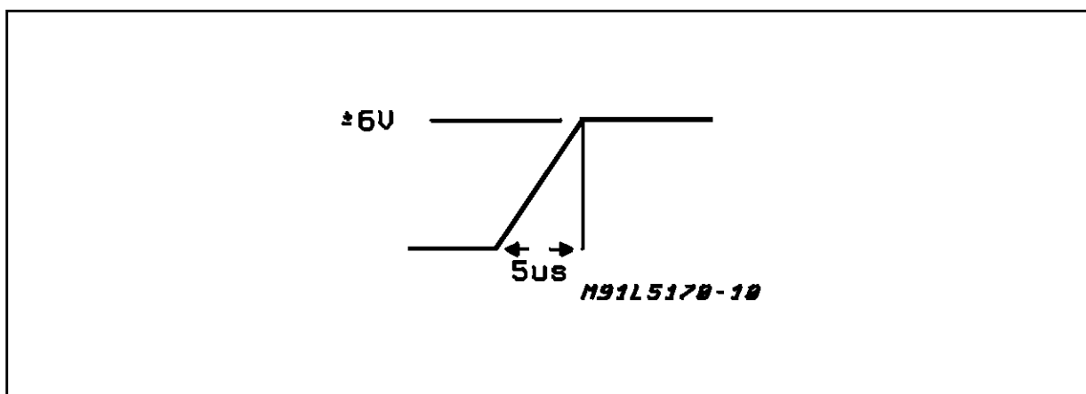
Figure 3: EOS Requirements
