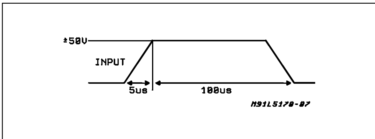
Figure 3: EOS Requirements
