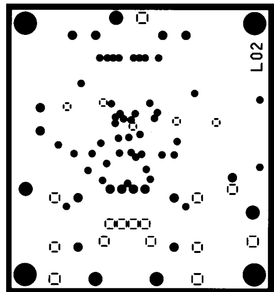
Signal Ground Plane
