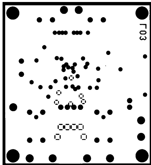
Power Ground Plane
