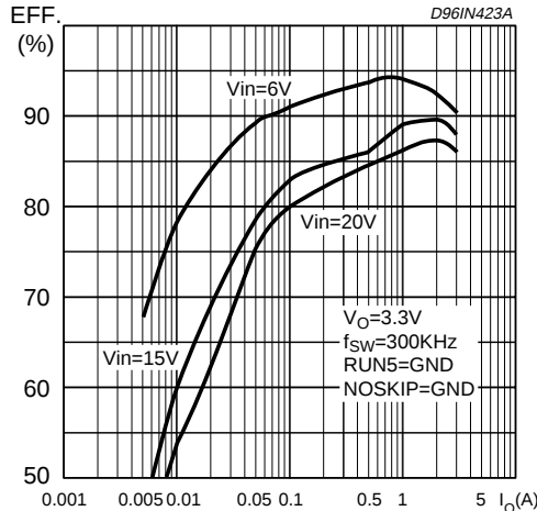
Figure 15: Demo Board Efficiency vs Output Current
