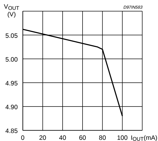
Figure 20: REG5 Regulator Characteristic ( V_{in} = 6V , RUN3 = RUN5 = LOW, T_j = 25^\circ C )
