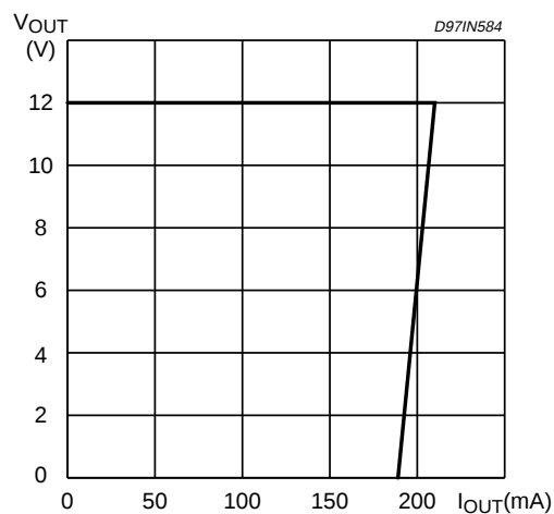
Figure 21: 12V Linear Regulator Characteristic ( V_{13IN} = 15V , RUN3 = HIGH, T_j = 25^\circ C )
