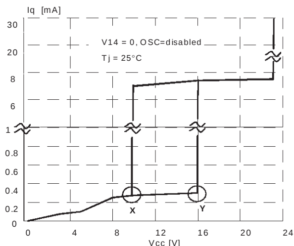
Figure 1. Quiescent current vs. input voltage. (X = 7.6V and Y = 8.4V for L4990A)
