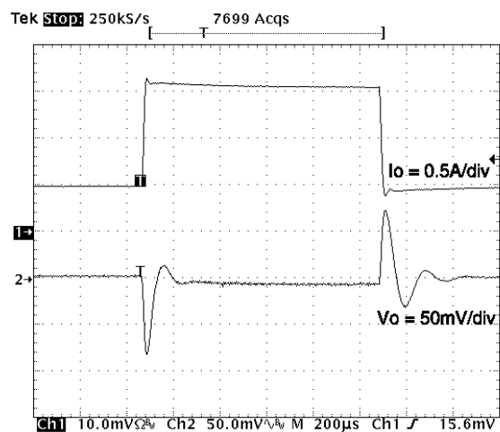
Figure 21. Load transient.
