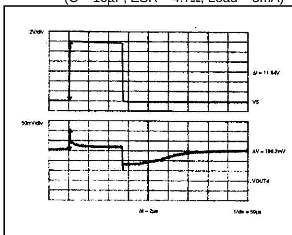
Figure 11: OUT4 supply transient response (C = 10 \mu F, ESR = 4.7 \Omega , Load = 3mA)
