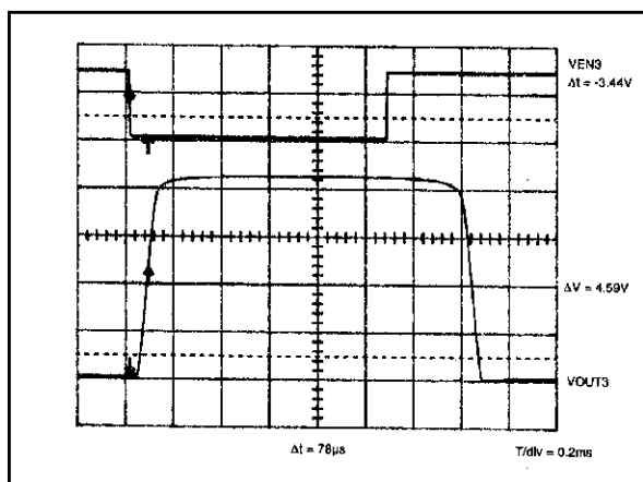
Figure 9: (C = 10 \mu F, ESR = 4.7 \Omega Load current 0mA and 117mA)
