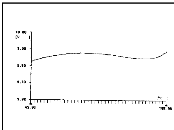
Figure 12: OUT4 voltage versus temperature
