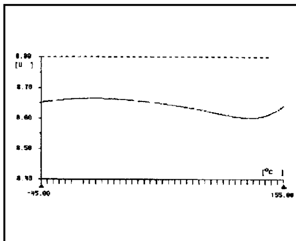
Figure 12: OUT4 voltage versus temperature
