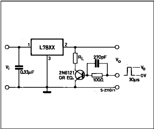
Figure 2 : Load Regulation.
